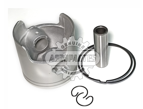
KIT PISTON 75 (0.50)
